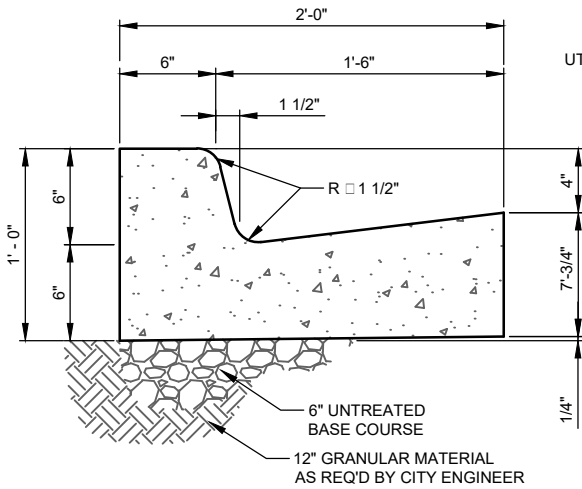
HIGH BACK CURB & GUTTER
