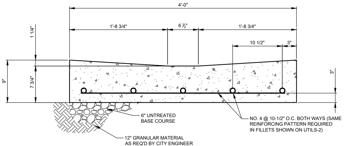
CROSS GUTTER
