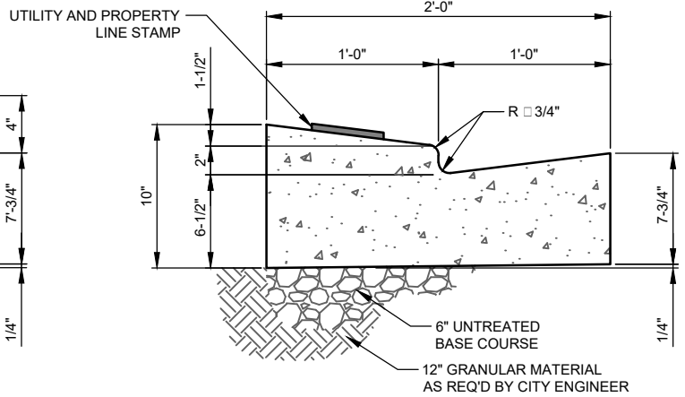
MODIFIED CURB & GUTTER
