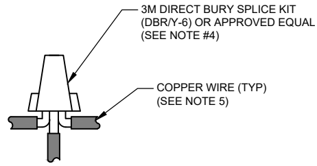
SPLICE DETAIL
